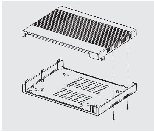
08-1: 47.5x280x200 08-1-1: 45.5x280x200 08-2: 35x140x110 08-3: 45x224x145 08-4: 65x260x180 08-8: 70x198x176 08-9: 80x205x230 08-10: 82x230x278
