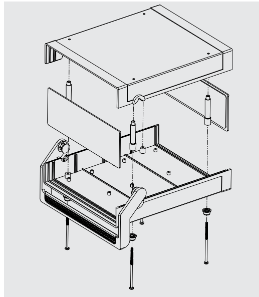
08-24-1: 53x100x150 08-25-1: 100x120x190 08-34: 108x290x258
