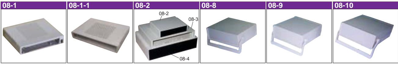
08-1: 47.5x280x200 08-1-1: 45.5x280x200 08-2: 35x140x110 08-3: 45x224x145 08-4: 65x260x180 08-8: 70x198x176 08-9: 80x205x230 08-10: 82x230x278
